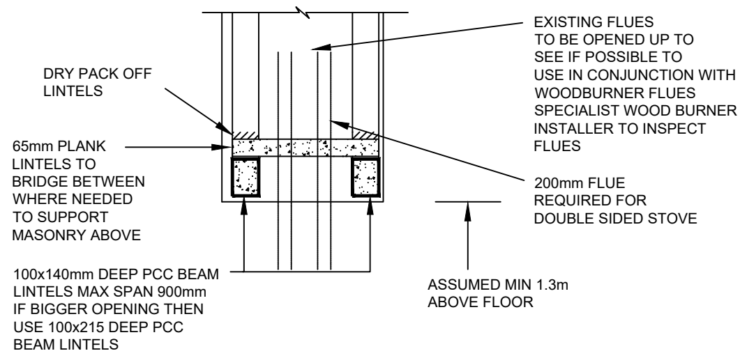
05,01 SECTION SCALE 1:20
